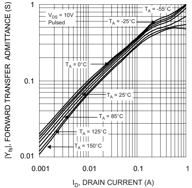
I_D , DRAIN CURRENT (A) Fig. 10 Forward Transfer Admittance vs. Drain Current
