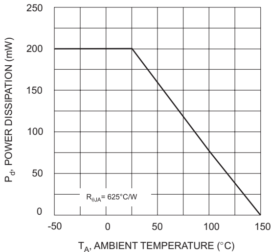
T_A , AMBIENT TEMPERATURE (°C) Fig. 11, Derating Curve - Total
